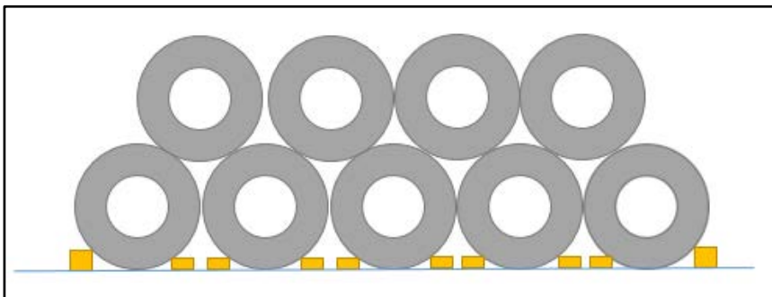
Correct Stowage of coils
